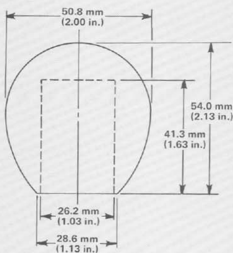
FIGURE 1 - Dimensions
